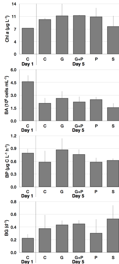
Figure 7. Planktonic variables in the 5-day experiment with amendments of glucose (G), glucose plus phosphorus (G + P), phosphorus (P), and palsa soil (S) to SAS1B lake water. The control (C) is shown on both day 1 and day 5. Each value is the mean \pm SD of triplicate samples.
